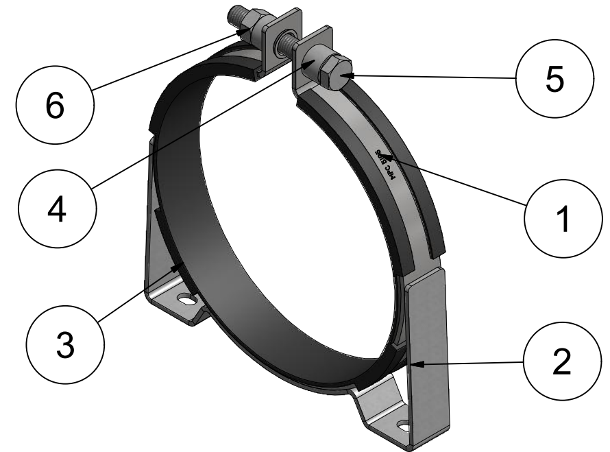
Parts identification ( 1 : 3 )
