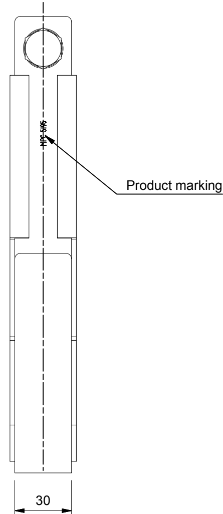
Side view ( 1 : 2 )
