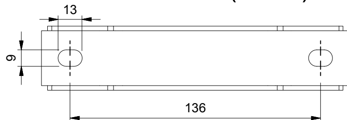
Bottom view ( 1 : 2 )
