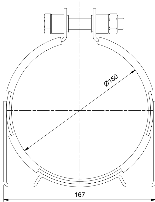
Front view ( 1 : 2 )
