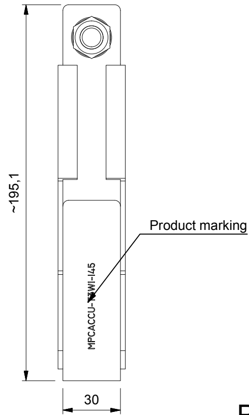
Side view ( 1 : 2 )
