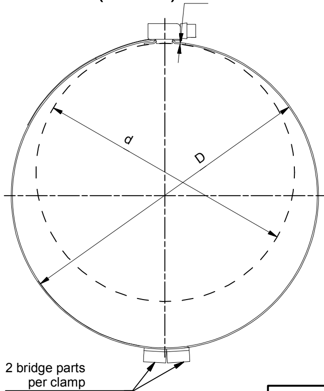
Front view ( 1 : 2 )
