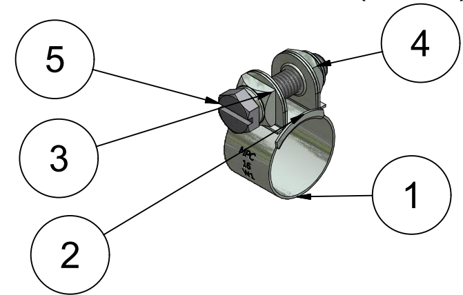
Parts identification ( 1 : 1 )
