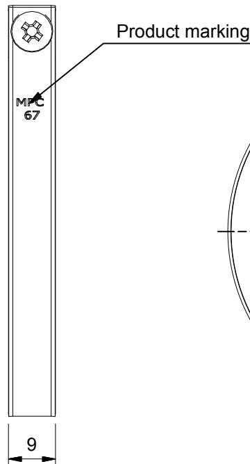
Side view ( 1 : 1 )
