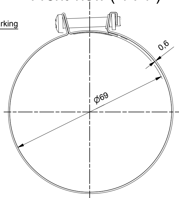
Front view ( 1 : 1 )
